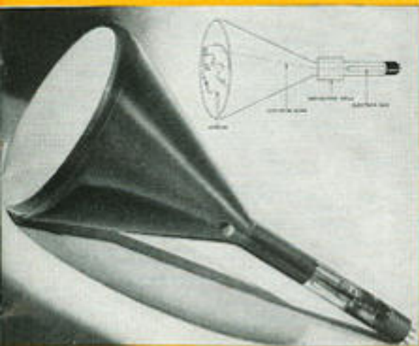
The Kinescope, corresponding to the "loud speaker" of an ordinary radio receiver. Diagram illustrates functioning.
