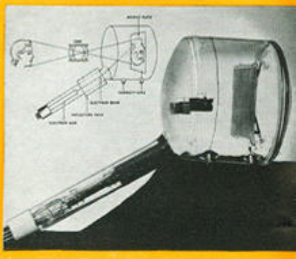
Iconoscope, the "electric eye" of the television camera. Diagram shows how lens focuses image on mosaic plate.
