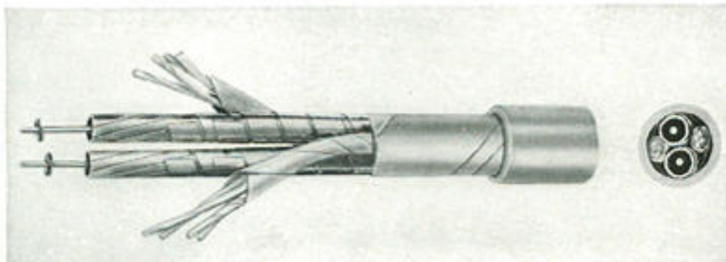
Photograph showing interior construction of coaxial cable used in television line transmission. Cross-section on right shows arrangement of essential parts. (Courtesy Bell Telephone Laboratories.)
