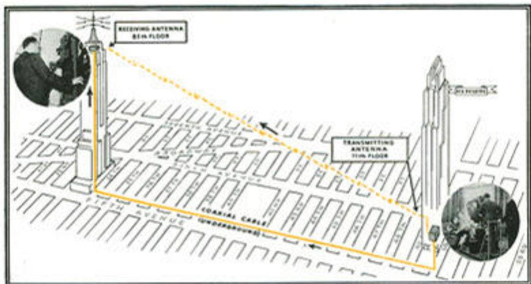
Sketch indicating how NBC television signals travel from RCA Building Studio 3H (right) to the Empire State Building transmitter (left). The solid yellow line represents a coaxial cable. Television picture signals may also be sent from studio to transmitter by radio waves, indicated by the broken yellow line.
