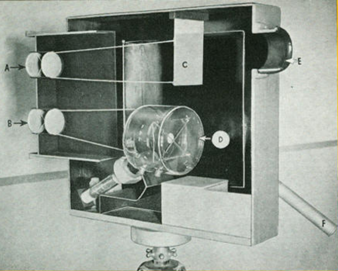
Simplified cutaway model of television studio camera, indicating principal parts. A—Focusing lens for ground-glass. B—Lens which focuses image on Iconoscope plate. C—Ground glass. D—Iconoscope. E—Viewing aperture which permits operator to see the ground-glass image. F—Focusing handle.
